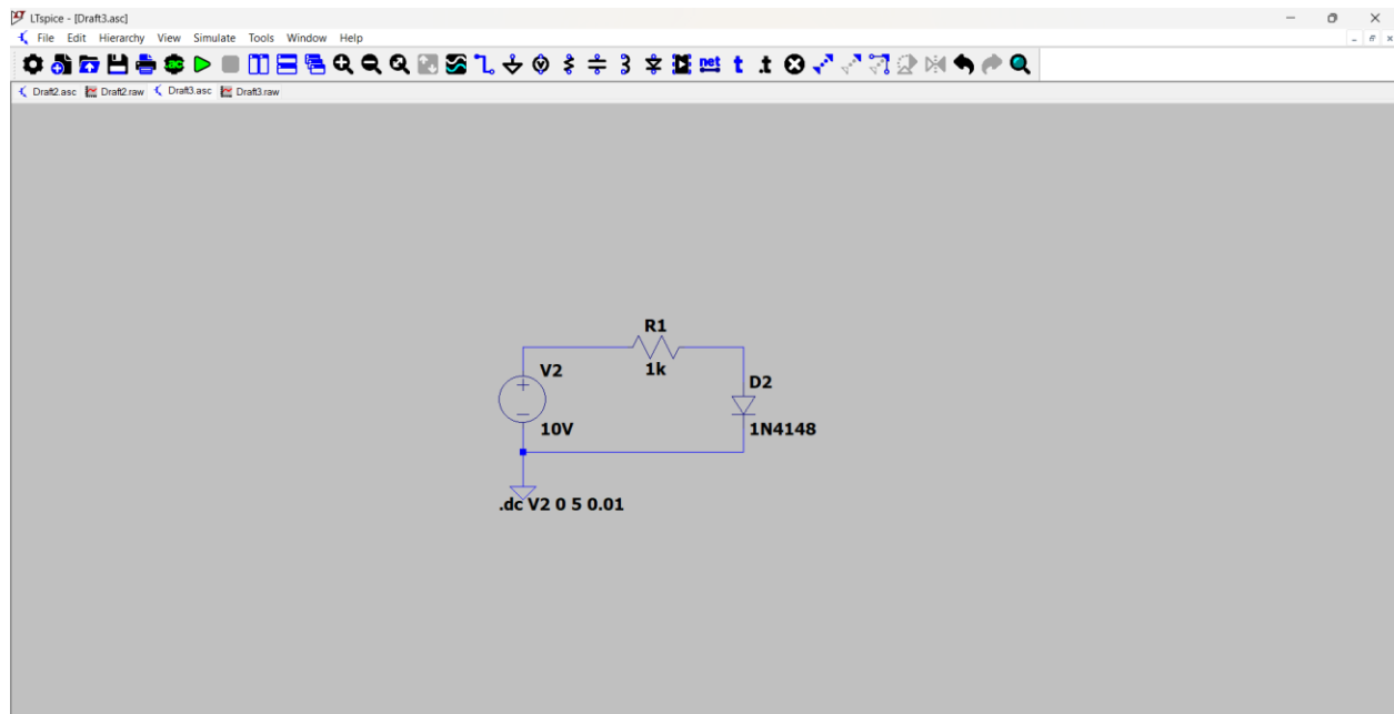
Figure 2: 1N4148 Diode Schematic View
